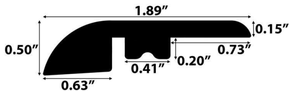
Reducer Olap WPC (290)
