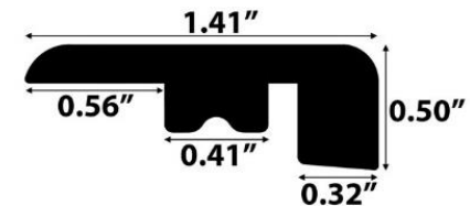
Square Nose WPC (291)
