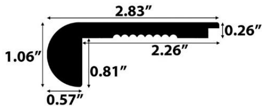
Stair Nose Flush WPC (288)
