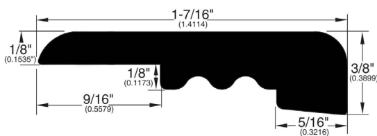
SQUARE NOSE WPC (300)
