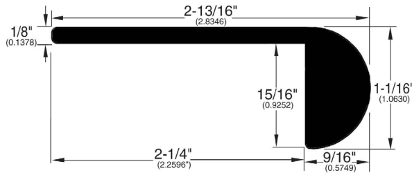
STAIR NOSE FLUSH WPC (298)
