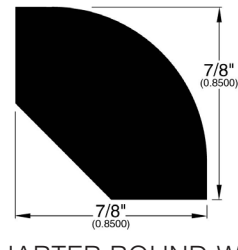
QUARTER ROUND WPC (296)
