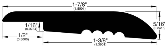
REDUCER OVERLAP WPC (297)
